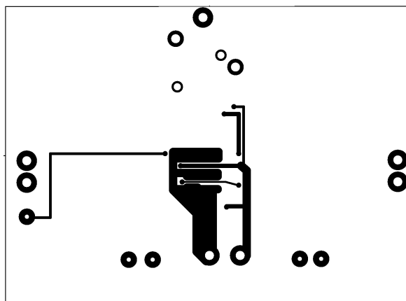
FIGURE 6. Recommended MTE PC board layout: bottom-side layout
