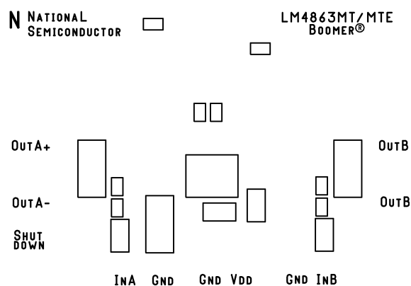
FIGURE 4. MTE PC board layout: Component-side Silkscreen
