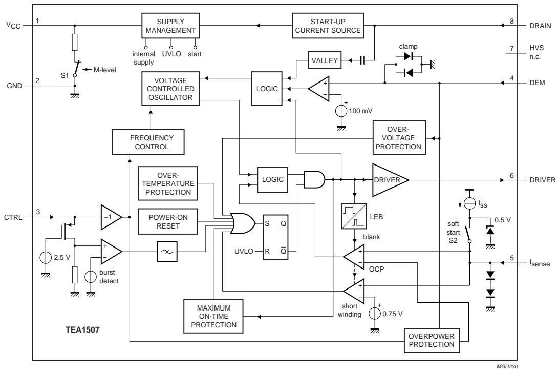
Fig.2 Block diagram.
