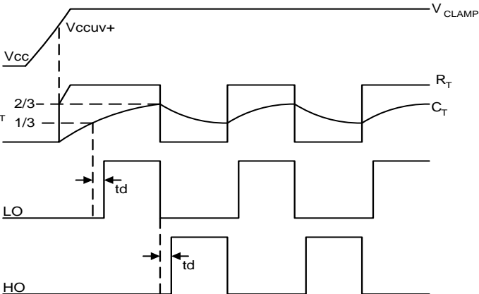
Figure 1. Input/Output Timing Diagram
