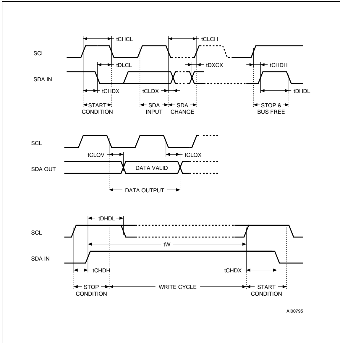
Figure 5. AC Waveforms
