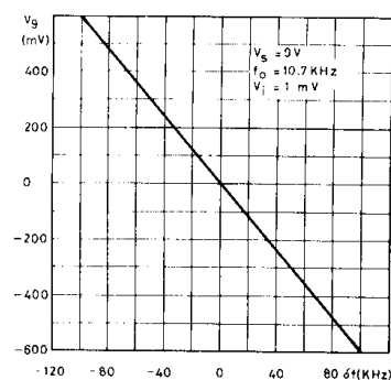
Figure 10. \Delta DC output voltage (pin. 9) vs. frequency shift (FM section)
