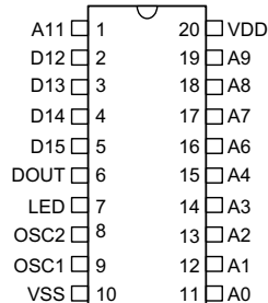
HT6207 - 20 DIP/SOP
