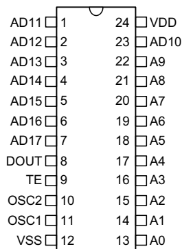
HT640 - 24 SOP/SDIP
