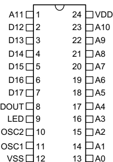
HT6247 - 24 SOP/SDIP
