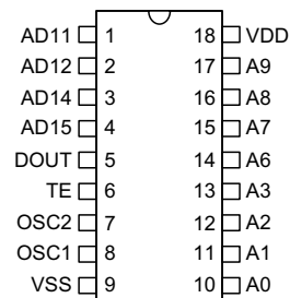
HT680 - 18 DIP/SOP
