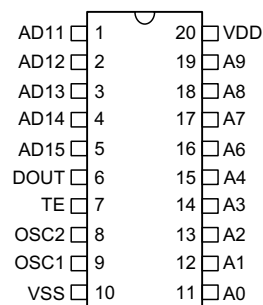
HT600 - 20 DIP/SOP
