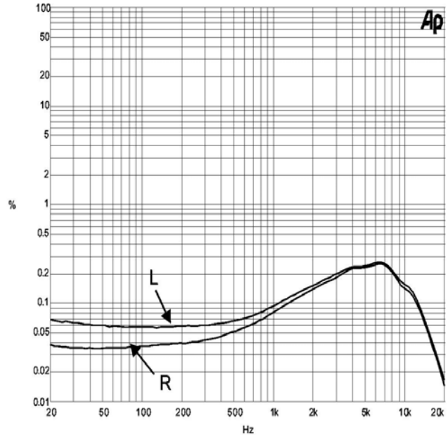
4. THD+N vs Frequency
