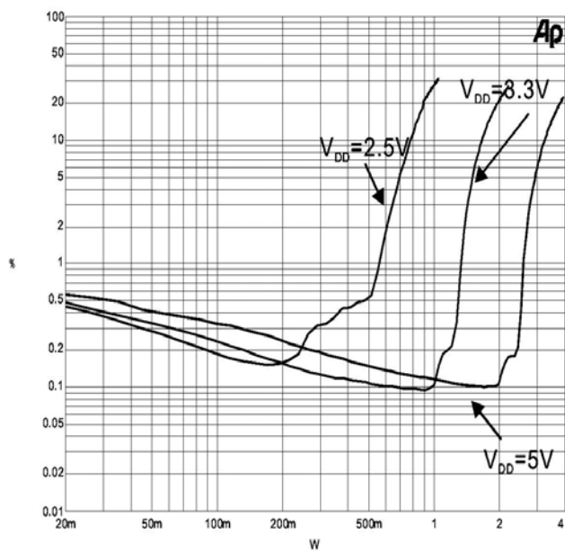
R L = 4Ω, Gain = 24dB, f = 1kHz
