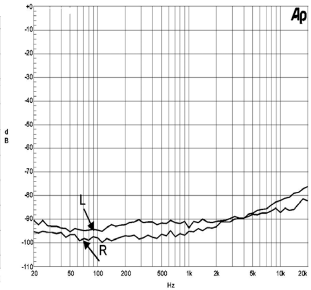
6. Crosstalk VS Frequency
