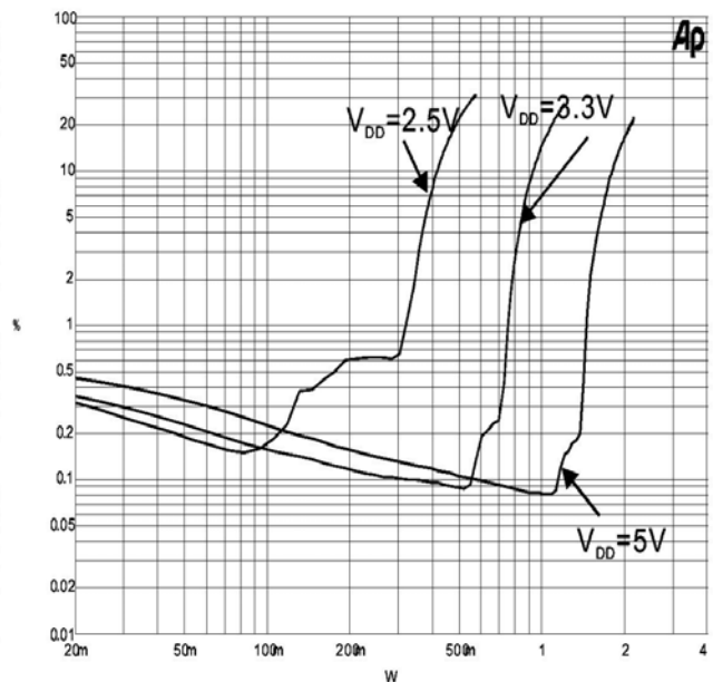
R L = 8Ω, Gain = 24dB, f = 1kHz
