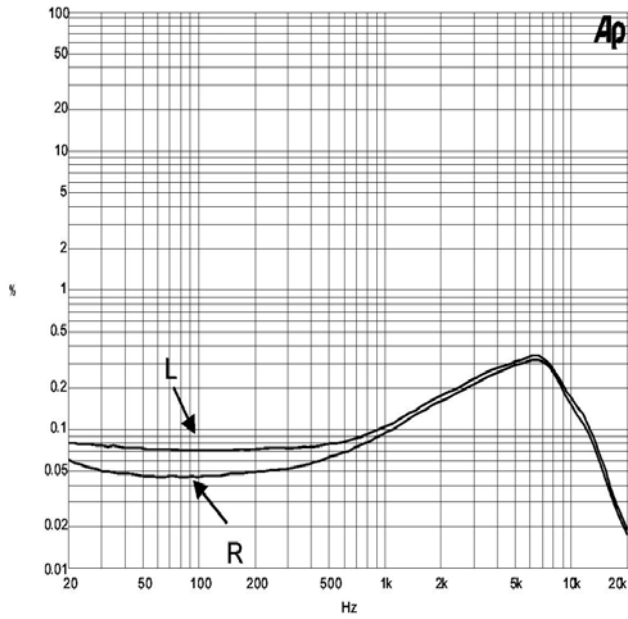
3. THD+N vs Frequency
