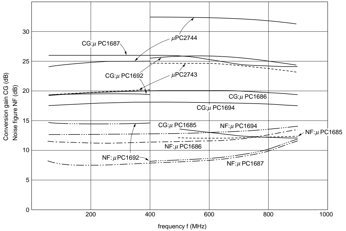
Conversion gain, noise figure vs. frequency
