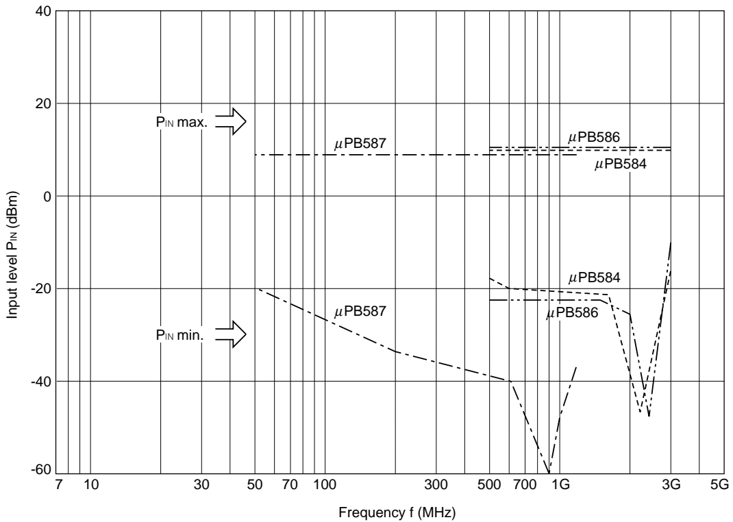
Input level vs. frequency
