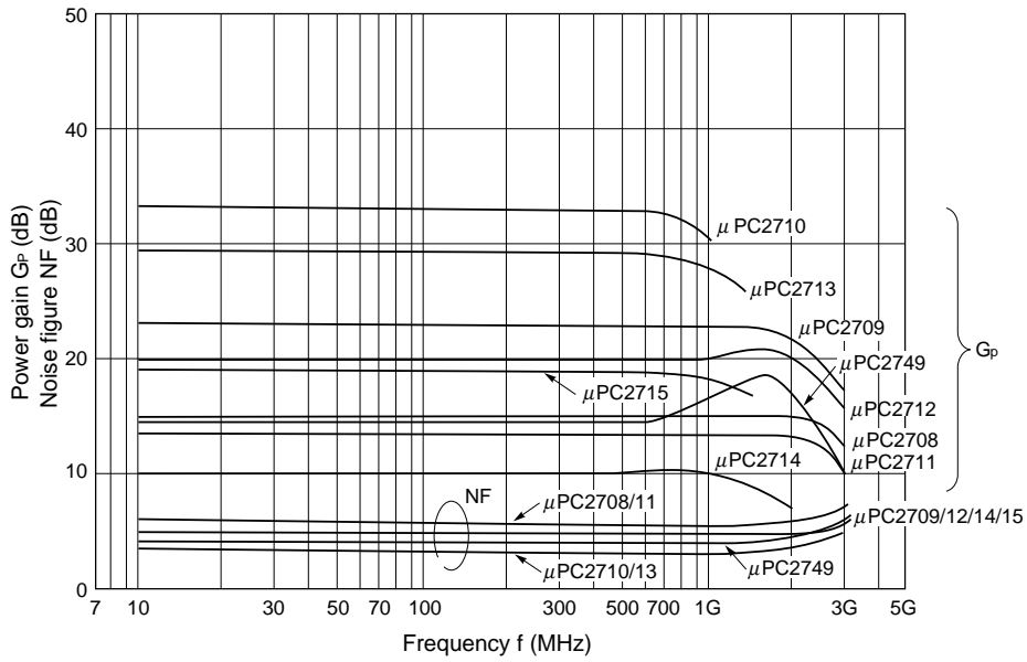
Power gain, noise figure vs. frequency
