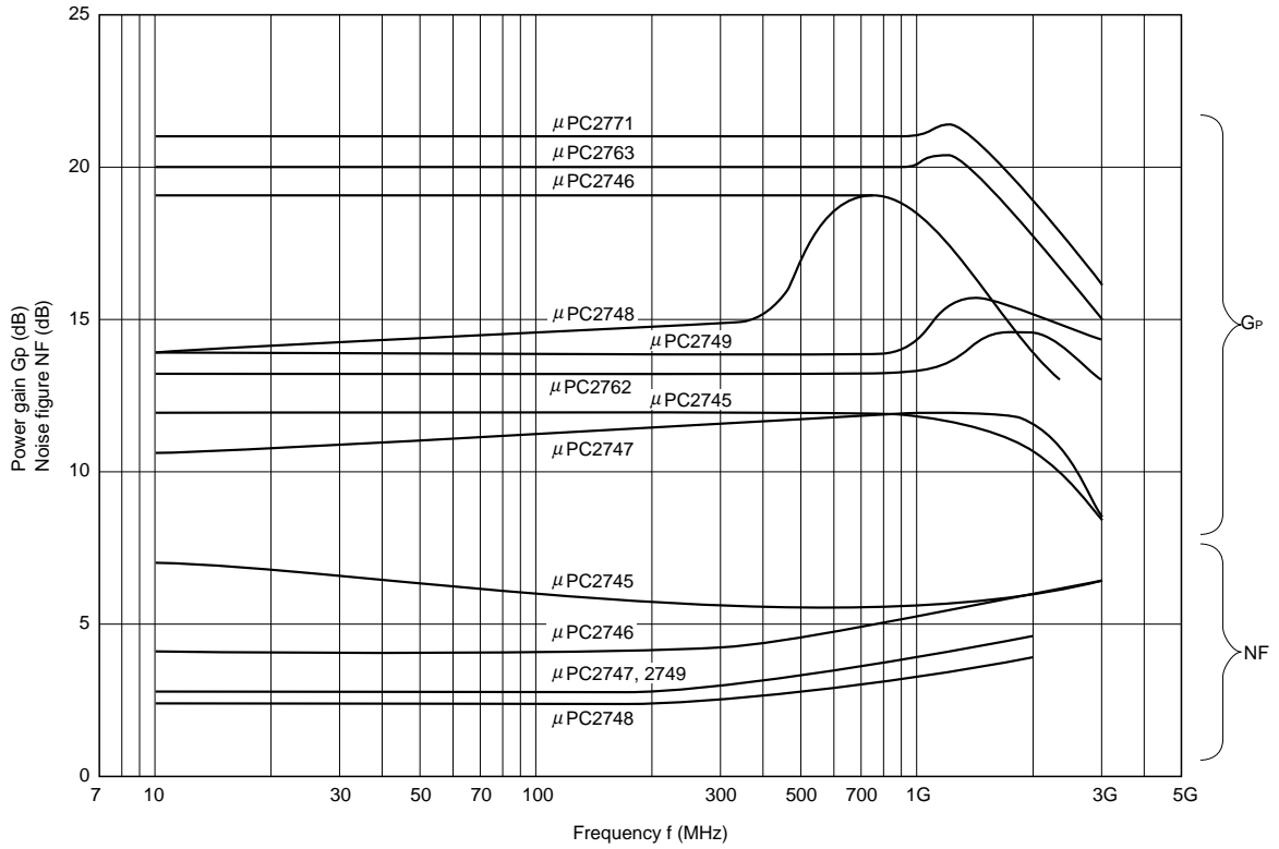
Power gain, noise figure vs. frequency
