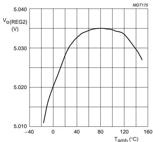
Fig.4 Output voltage of regulator 2 as a function of the ambient temperature.
