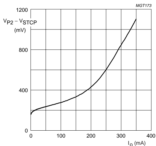
Fig.5 Voltage drop of V_{P2} as a function of the output current of regulator 2.
