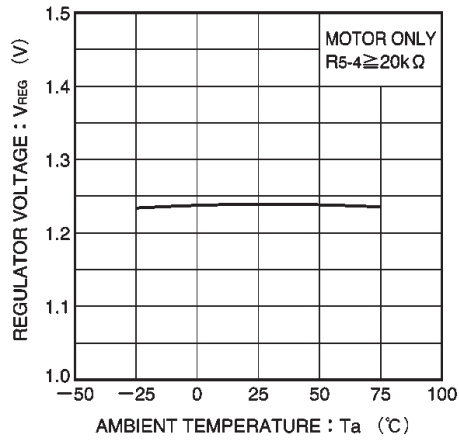
Fig. 28 Regulator voltage vs. ambient temperature
