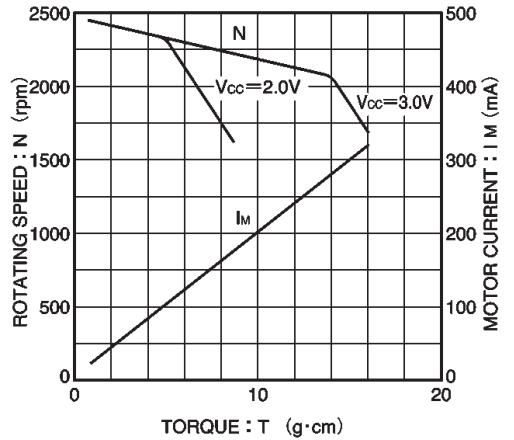
Fig. 29 Rotation speed and motor current vs. torque
