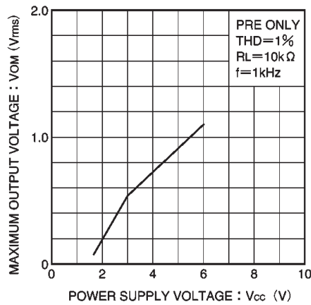
Fig. 22 Maximum output voltage vs. power supply voltage
