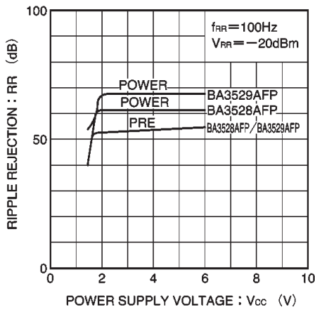
Fig. 21 Ripple rejection ratio vs. power supply voltage
