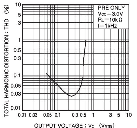
Fig. 23 Total harmonic distortion vs. output voltage
