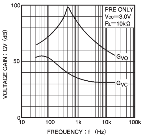
Fig. 24 Voltage gain vs. frequency
