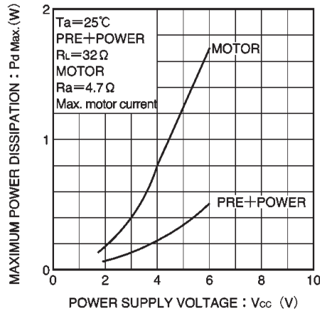
Fig. 19 Maximum power dissipation vs. power supply voltage
