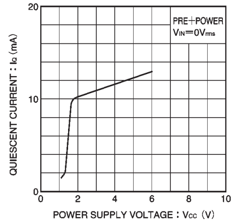
Fig. 20 Quiescent current vs. power supply voltage
