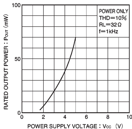
Fig. 25 Rated output power vs. power supply voltage
