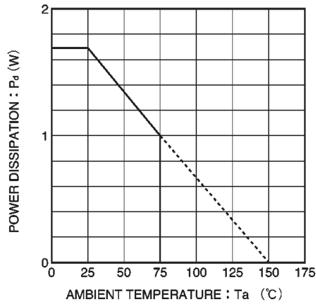
Fig. 18 Power dissipation vs. ambient temperature
