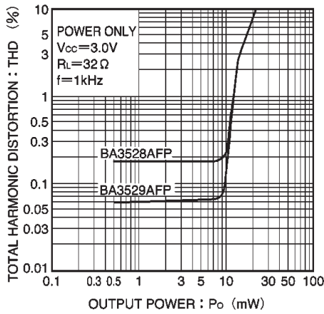
Fig. 27 Total harmonic distortion vs. output voltage
