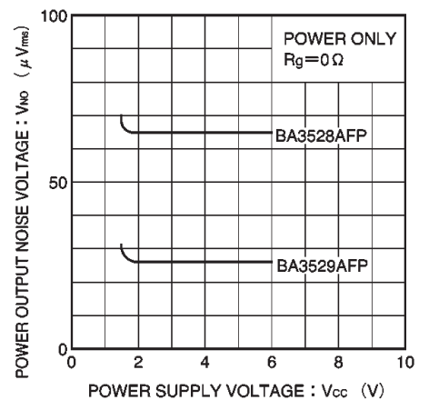
Fig. 26 Output noise voltage vs. power supply voltage
