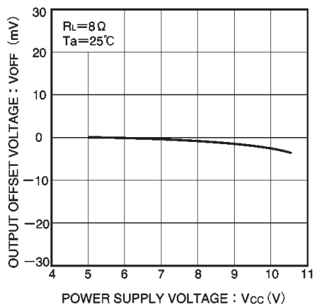
Fig. 9 Power supply voltage vs. output voltage (offset)
