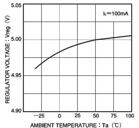
Fig. 11 Regulator voltage vs. temperature
