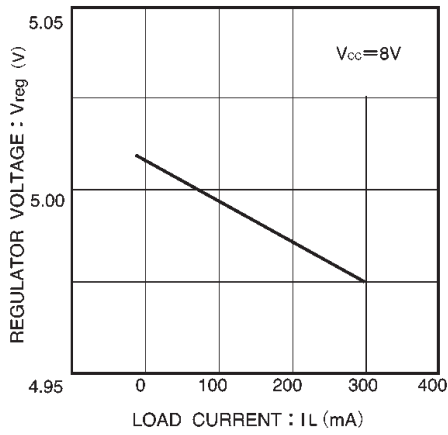
Fig. 12 Load current vs. regulator current
