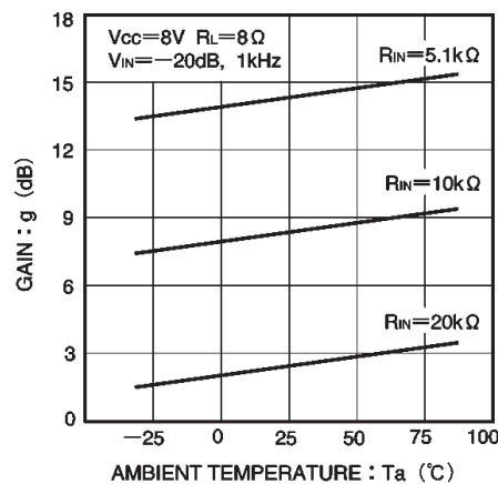
Fig. 10 Driver gain vs. temperature (Rin connected via gain adjustment pin)
