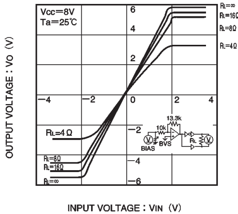
Fig. 7 Driver I/O characteristics (variable load)
