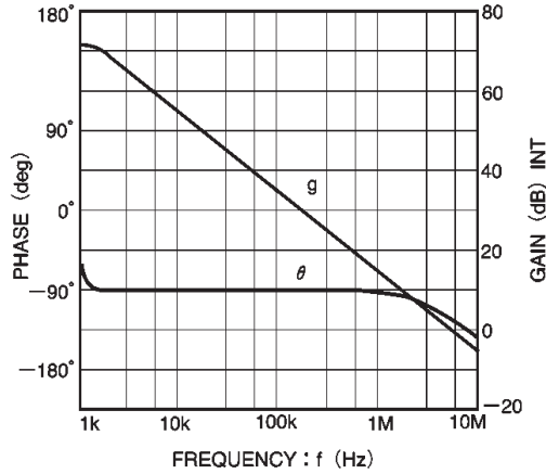
Fig. 13 Operational amplifier vs. open loop
