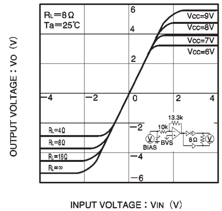
Fig. 8 Driver I/O characteristics (variable Vcc)
