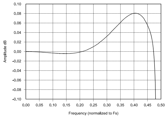
Figure 18. Passband Ripple
