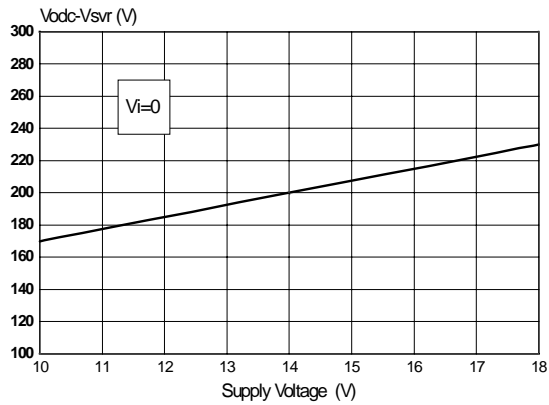
Output DC Offset vs. Supply Voltage
