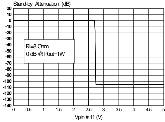
St-By Attenuation vs. Vpin 11
