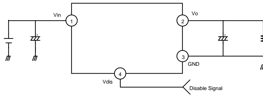
Figure 1. Application Circuit
