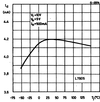
Figure 13: Quiescent Current vs Junction Temperature
