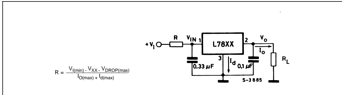
Figure 33: Remote Shutdown
