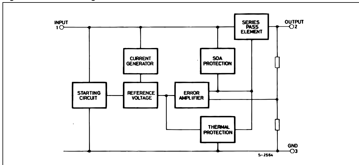
Figure 1: Schematic Diagram
