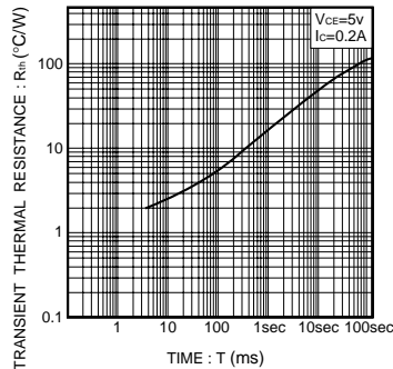
Fig.11 Transient thermal resistance (2SD1760)
