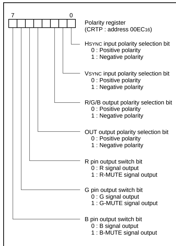
Fig. 33 Structure of CRT port control register
