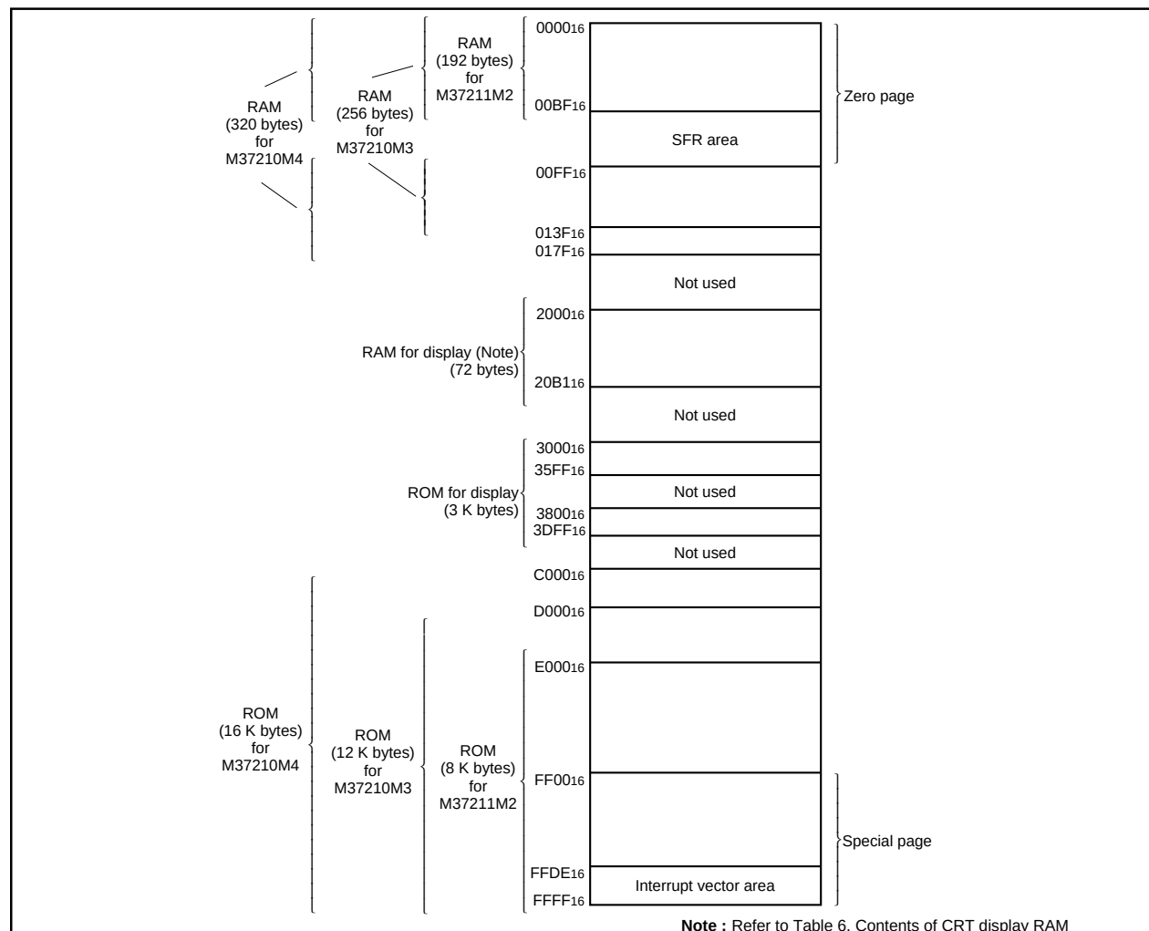
Fig. 2 Memory map
