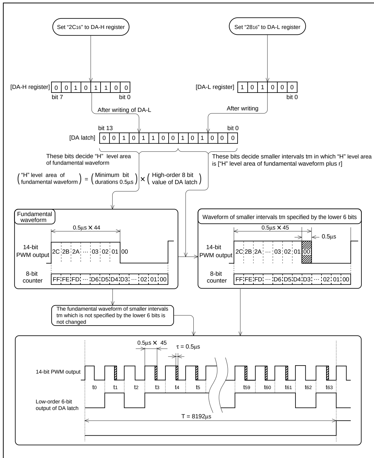
Fig. 14 14-bit PWM output example ( f(X_{IN}) = 4\text{MHz} )
