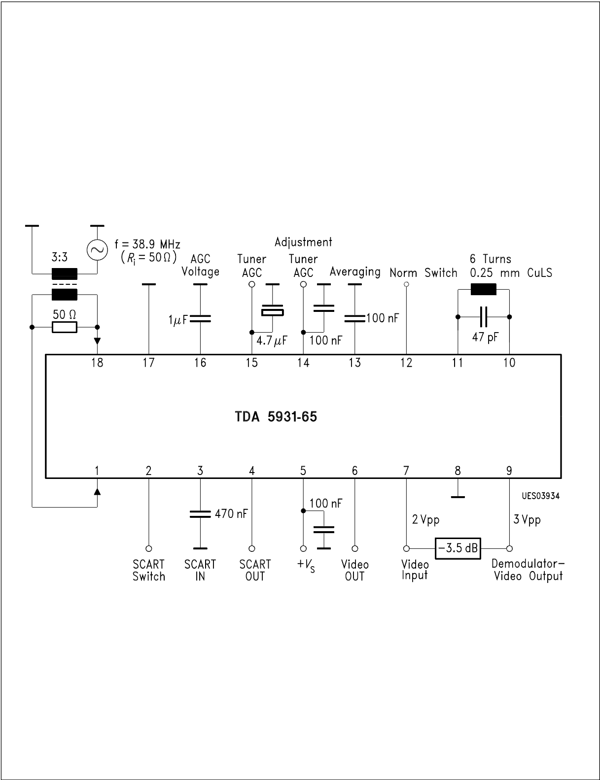
Test Circuit
