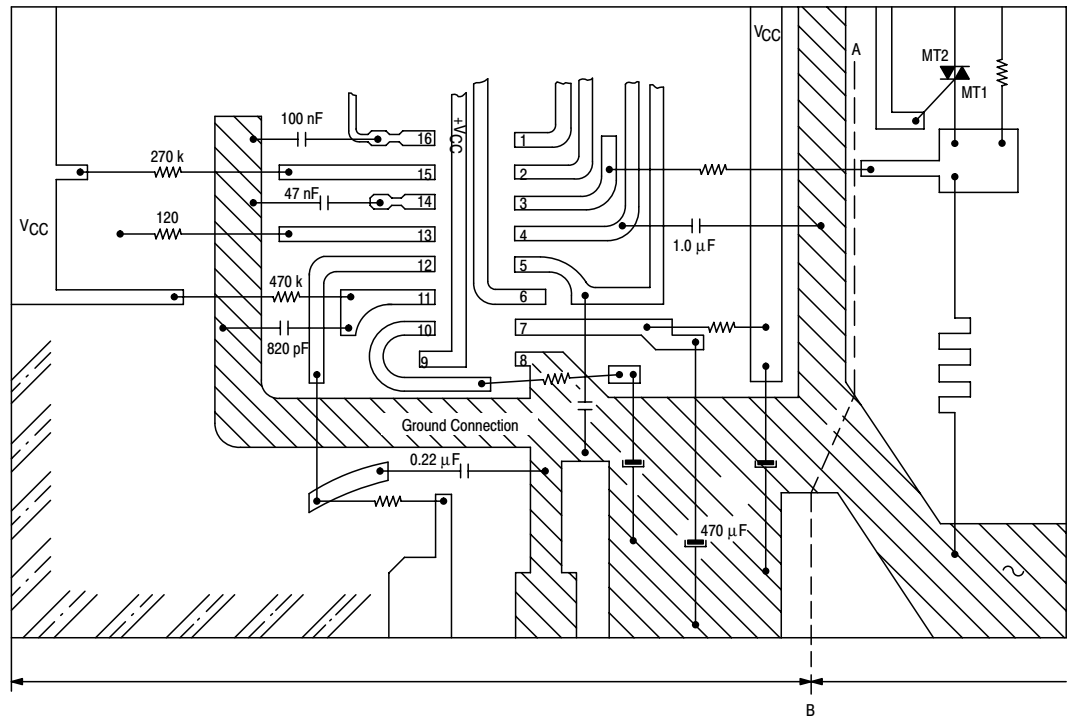
Figure 5. PC Board Layout
