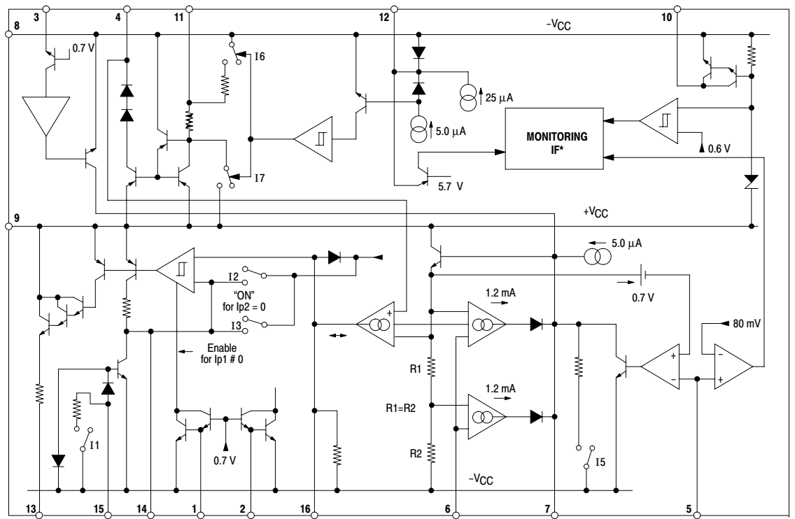
Figure 8. Simplified Schematic
