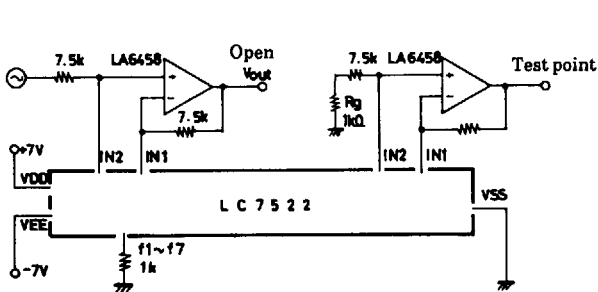
Test Circuit 2
